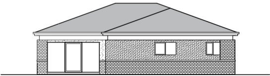
Typical North Elevation
